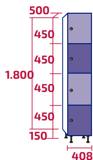
AMC400/1 COD: 10453 | 10502 42kg | 45kg - 0,37m 3
