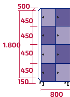
AMC300/2 COD: 10450 | 10499 64kg | 68kg - 0,54m 3
