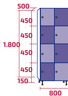
AMC400/2 COD: 10454 | 10503 74kg | 79kg - 0,72m 3
