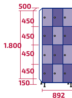
AMC300/3 COD: 10451 | 10500 91kg | 97kg - 0,80m 3
