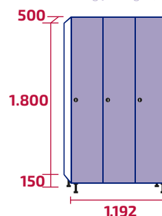
AMV400/3 COD: 10434 | 10483 89kg | 97kg · 1,07m 3
