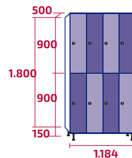
AMT300/4 COD: 10438 | 10487 101kg | 110kg · 1,07m 3
