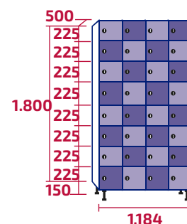
AMZ300/4 COD: 10473 | 10522 152kg | 160kg · 1,07m 3
