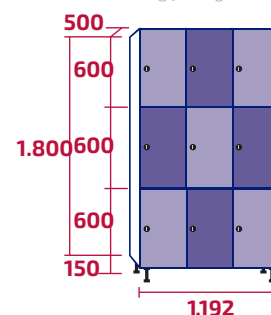
AMM400/3 COD: 10448 | 10497 98kg | 107kg - 1,07m 3
