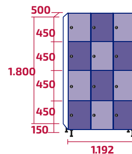
AMC400/3 COD: 10455 | 10504 106kg | 115kg - 1,07m 3
