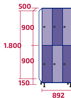
AMT300/3 COD: 10437 | 10486 78kg | 85kg · 0,80m 3
