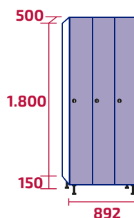
AMV300/3 COD: 10430 | 10479 77kg | 83kg · 0,80m 3
