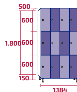
AMM300/4 COD: 10445 | 10494 110kg | 118kg - 1,07m 3
