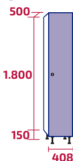
AMV400/1 COD: 10432 | 10481 36kg | 37kg · 0,37m 3
