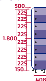
AMZ400/1 COD: 10474 | 10523 52kg | 55kg · 0,37m 3
