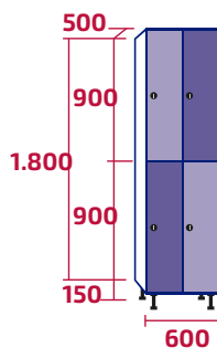
AMT300/2 COD: 10436 | 10485 55kg | 60kg · 0,54m 3
