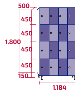
AMC300/4 COD: 10452 | 10501 118kg | 127kg - 1,07m 3
