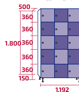
AMP400/3 COD: 10462 | 10511 114kg | 123kg · 1,07m 3
